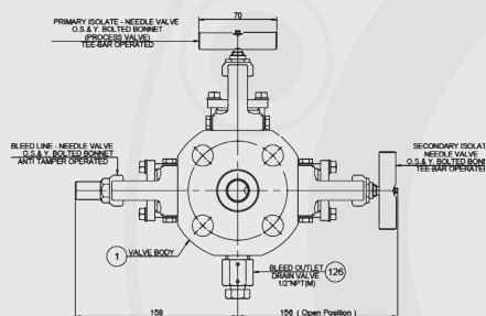
Monoflange (Slimline)
