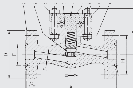
Check - Piston
