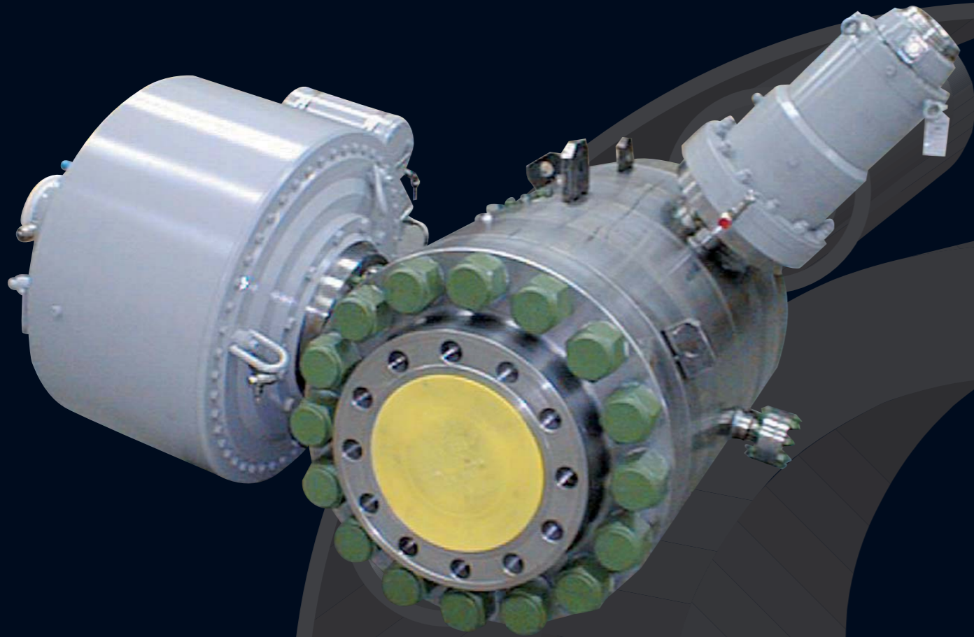
12" 2500# F65 SUBSEA FULL BORE PIGGABLE
