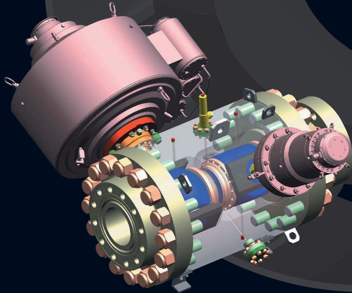
12" 2500# F65 SUBSEA FULL BORE PIGGABLE
